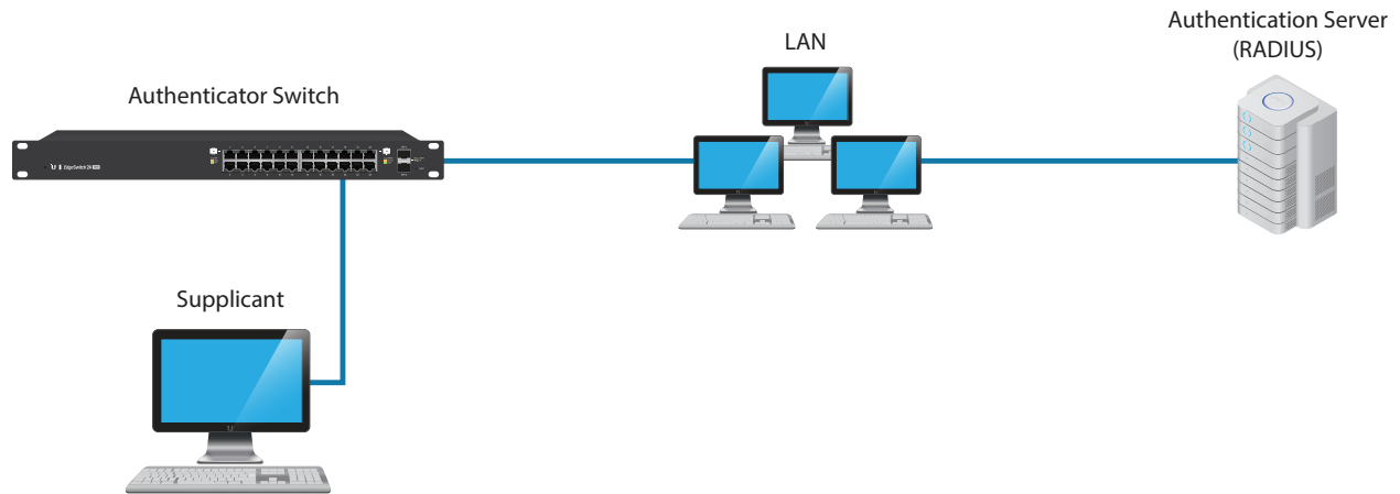
Switch with 802.1X Network Access Control
