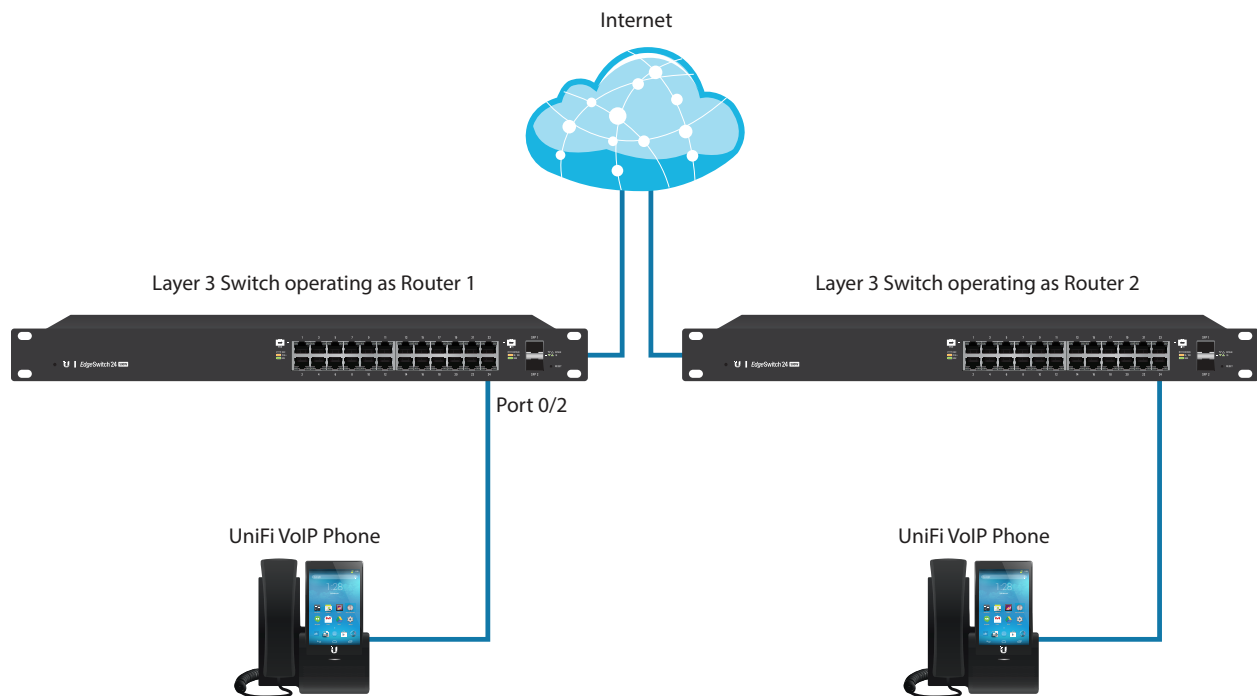
DiffServ VoIP Example Network Diagram
